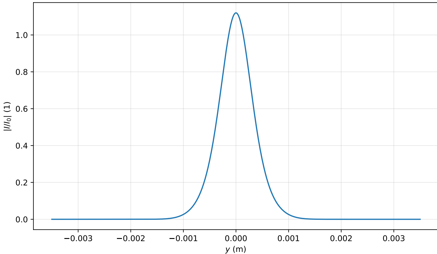
Intensity profile I(x=0, y, z=1.035)/I_0 , P_{in}=0.6P_{cr} , artificial time
